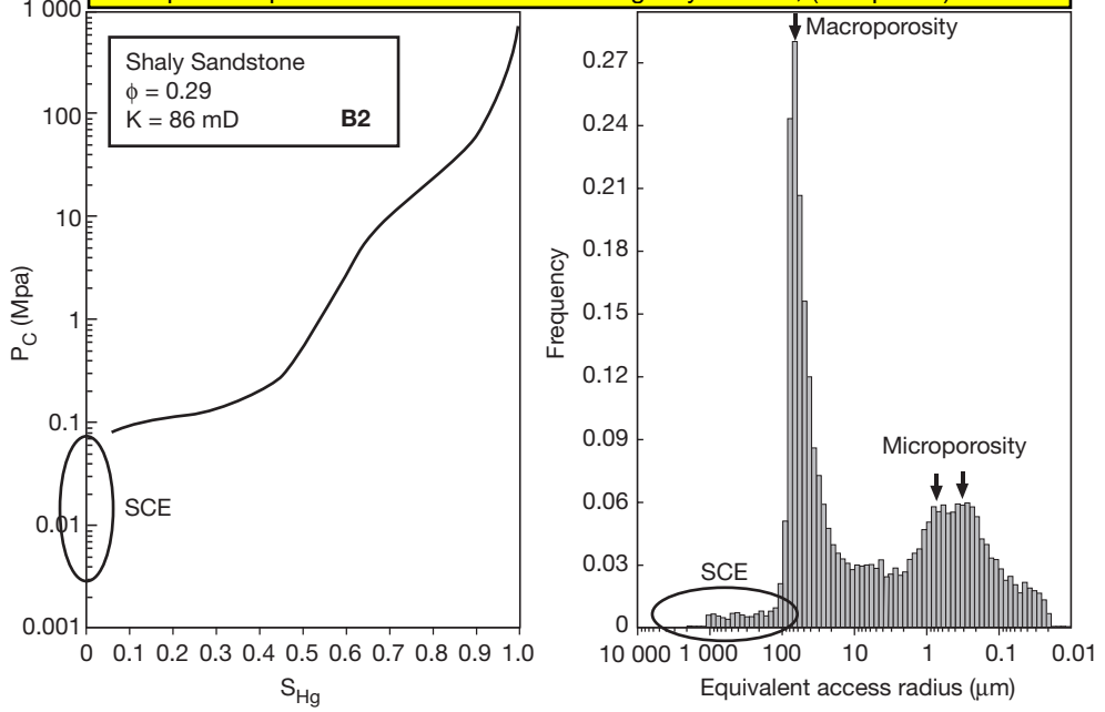
Figure 1-1.46 Example of application of porosimetry to the quantitative description of the porous space of sandstone of increasing clay content; (four plates)
