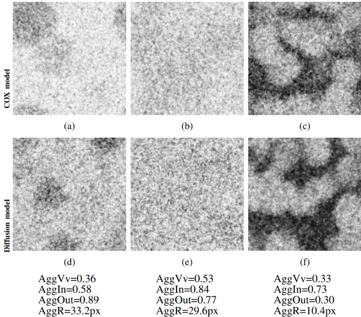
Fig. 1: COX model-generated (a–c) vs. diffusion-generated microstructures (d–f).
